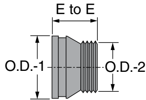
FIGURE 7076 CONCENTRIC REDUCER (GROOVE BY THREAD)
